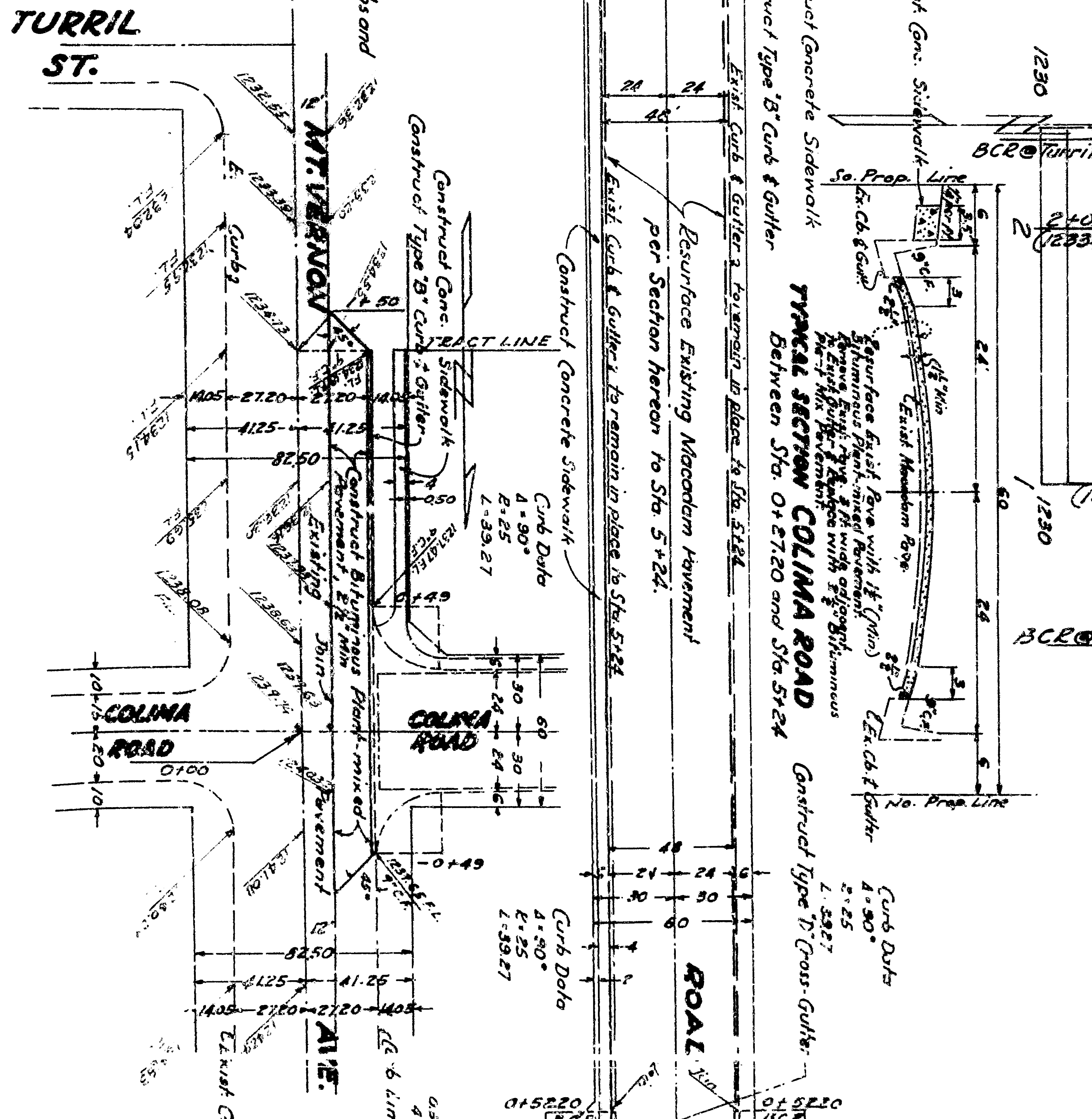
PLANS Scale 1" = 40'
